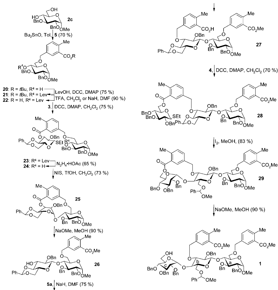
Scheme 5. Synthesis of target molecule 1
