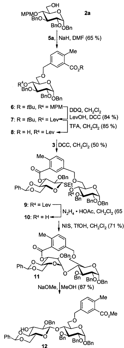
Scheme 3. Synthesis of disaccharide 12 with a 3-(methoxycarbonyl)benzyl spacer
