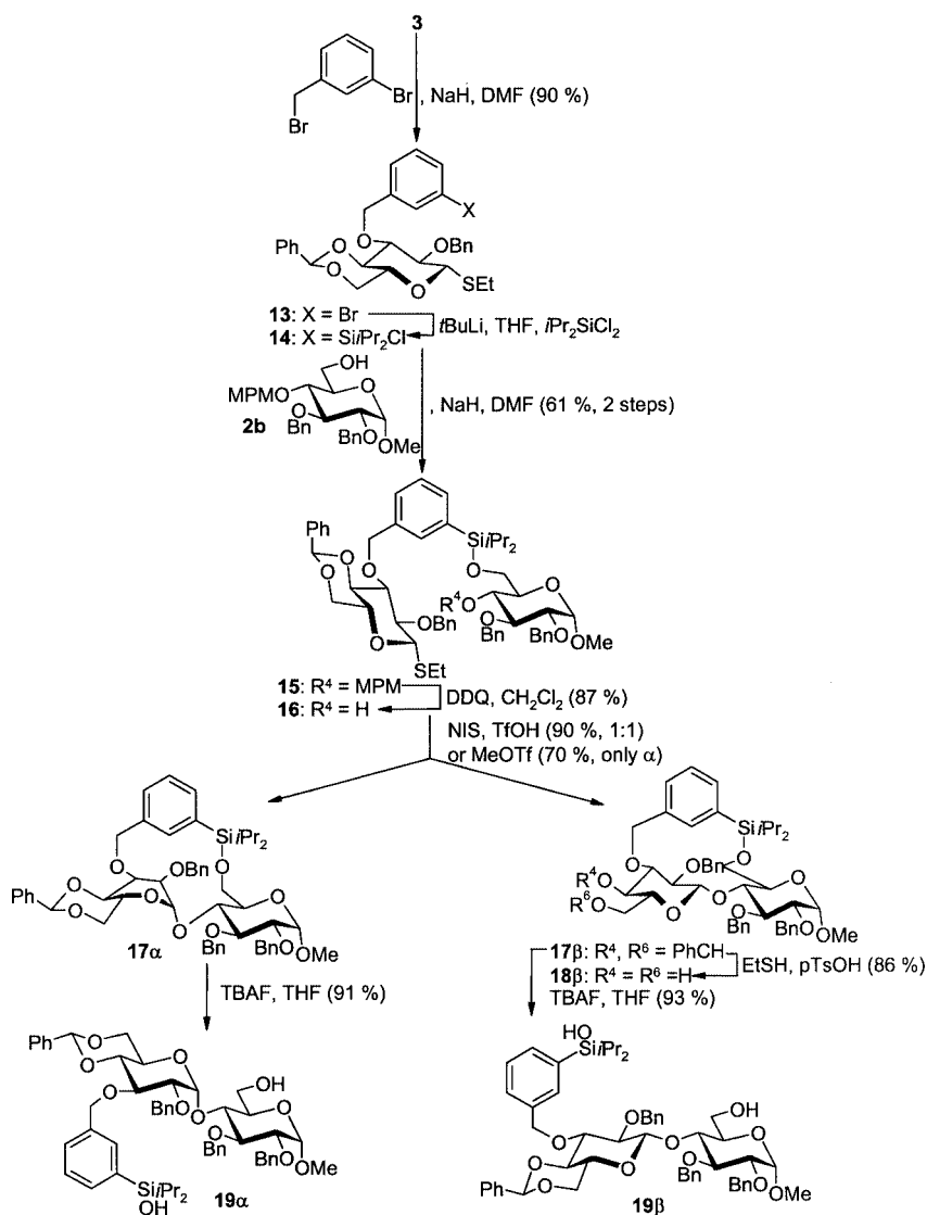
Scheme 4. Synthesis of disaccharides 19 with a 3-silylbenzyl spacer
