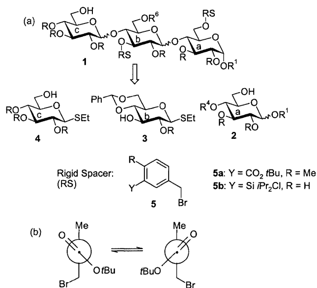
Scheme 2. (a) Retrosynthesis of target molecule 1 ; (b) preferred conformers of 5a ; R = Bn; R 1 = Bn, Me; R 4 = MPM, H; R 6 = PhCHOMe; RS = rigid spacer
