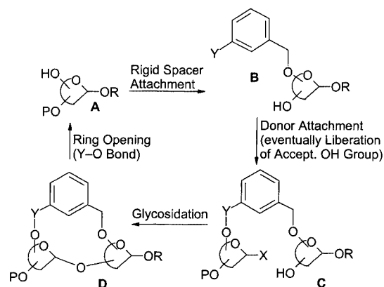
Scheme 1. Reiterative intramolecular oligosaccharide synthesis, R increasing with each cycle
